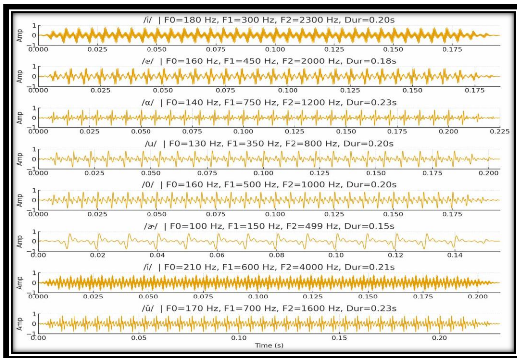
Figure (2) the formants description of some Kurdish vowels
