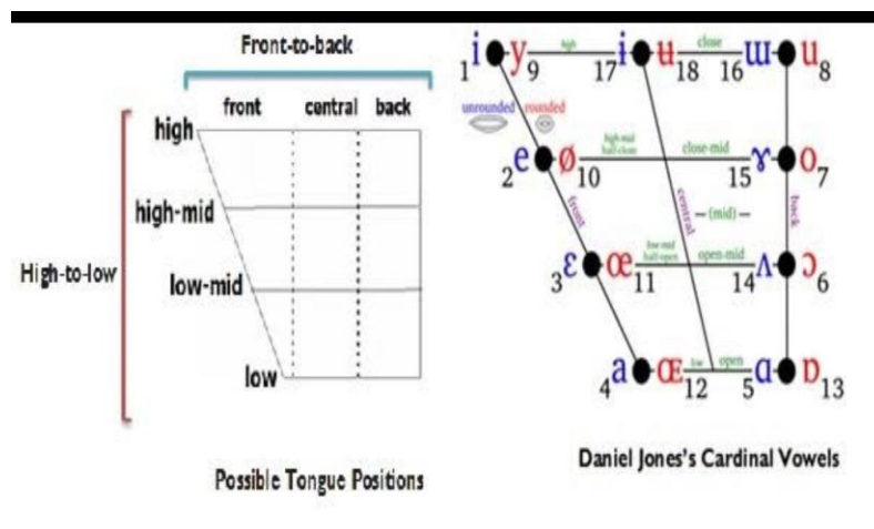
Figure (1) IPA vowel chart
